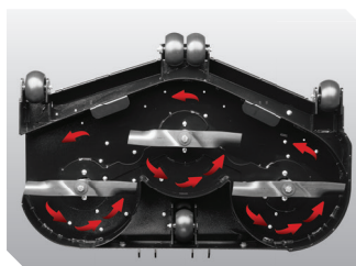
60" and 72" Decks – Deep 7 gauge shell to tackle deep grass with ease
